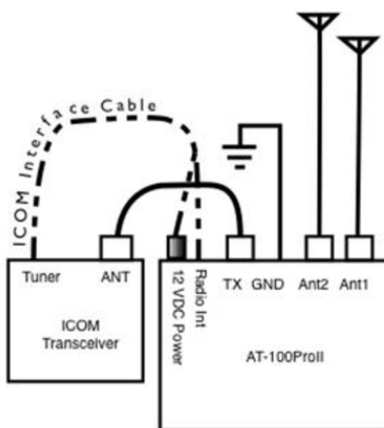
ICOM Installation
