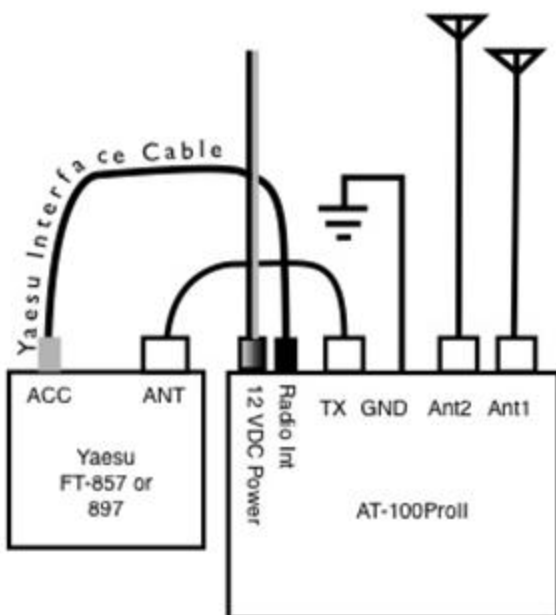
FT-857/897 Installation
